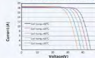
I-V CURVES OF PV MODULE(650W)
