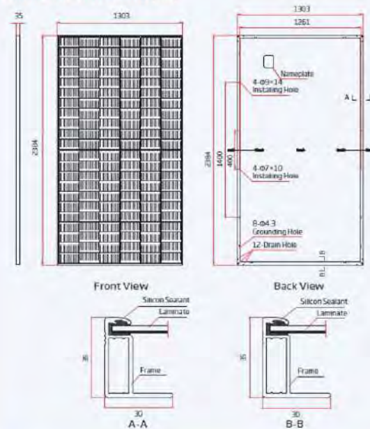
DIMENSIONS OF PV MODULE(mm)
